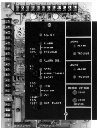
FS2000 Basic control module
