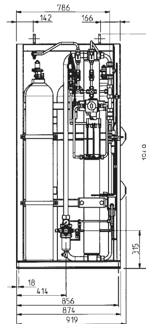
Left end view
